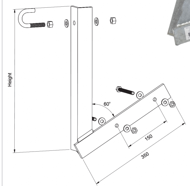
(Schematic Diagram)
